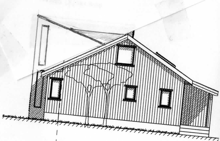
Fasade N/V
