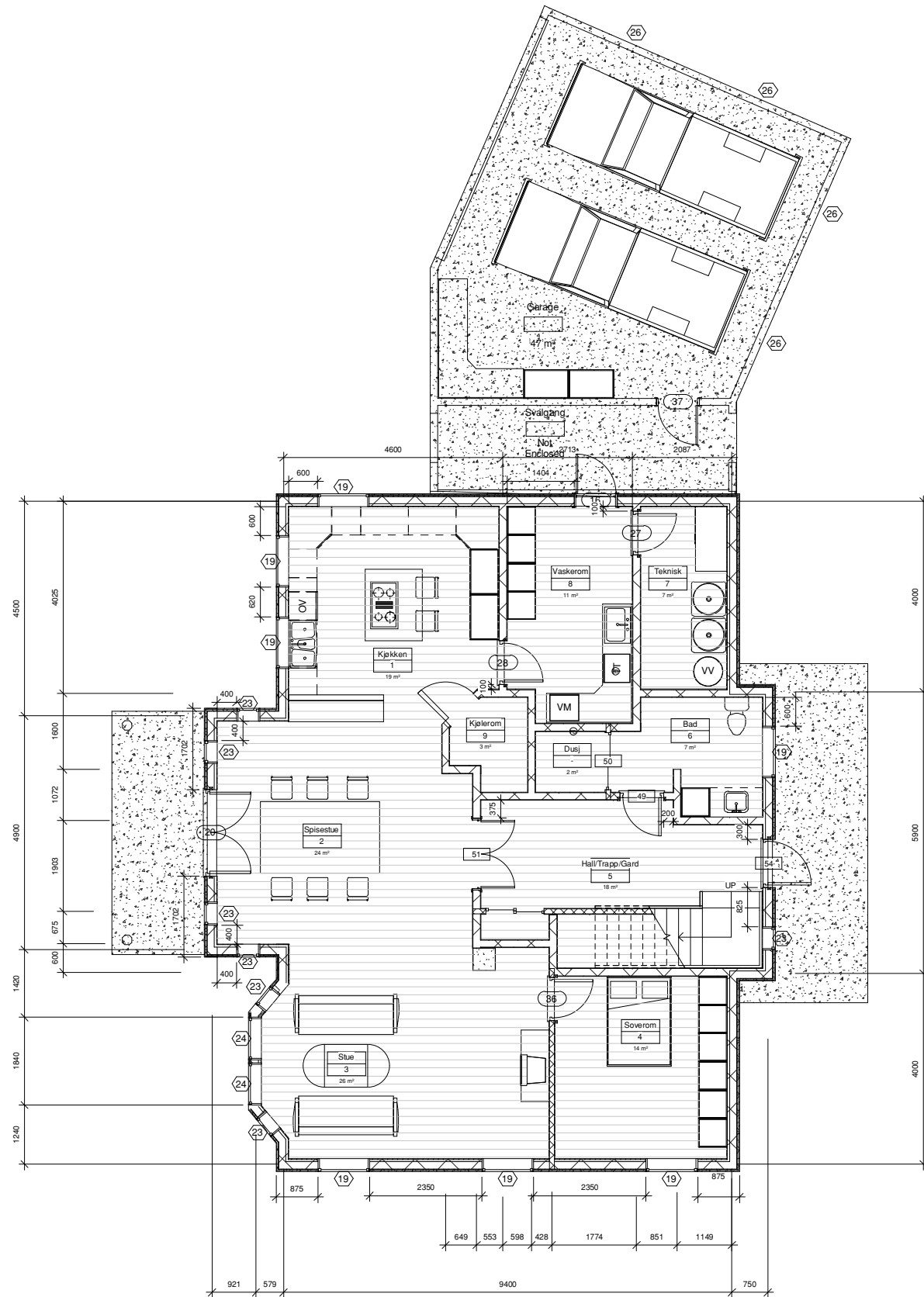
1 Grunnplan 1 : 50
